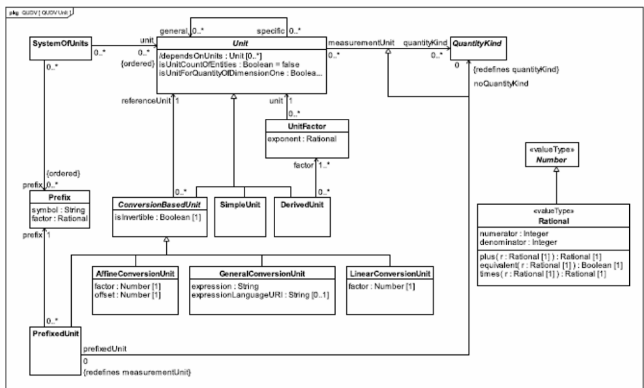
Figure E.6 - QUDV Units diagram
