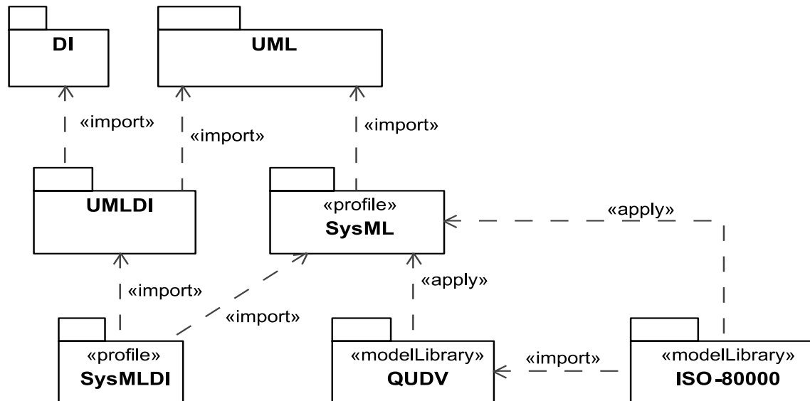
Figure 4.4 - Non-normative Package Structure
